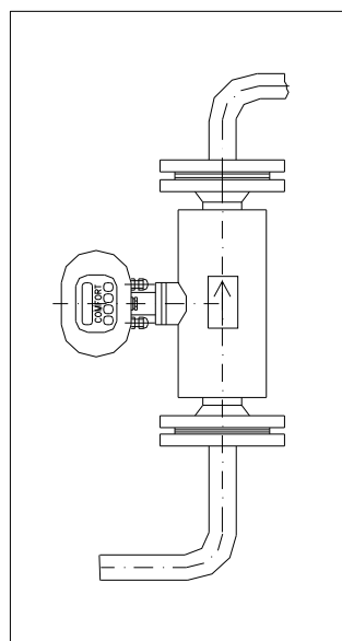
Sensor installed in a vertical section of the fluid piping
