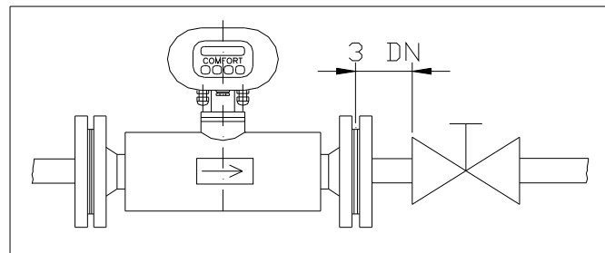
Required straight piping section for a “disturbance” located at the sensor output
